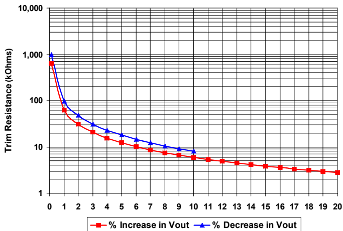
Figure C: Trim Graph for 2.0V out module
