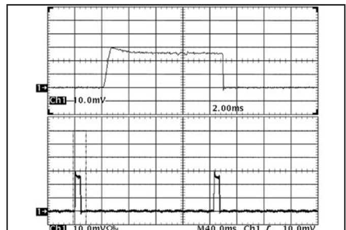
Figure 18: Load current ( 20\ \text{A}/\text{div} ) as a function of time when the converter attempts to turn on into a 1\ \text{m}\Omega short circuit. Top trace ( 2\ \text{ms}/\text{div} ) is an expansion of the on-time portion of the bottom trace.
